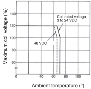
Ambient Temperature vs. Maximum Coil Voltage G5V-2
